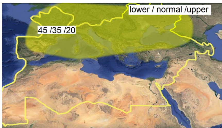
Figure 2. The same as figure 1 but for precipitation.
