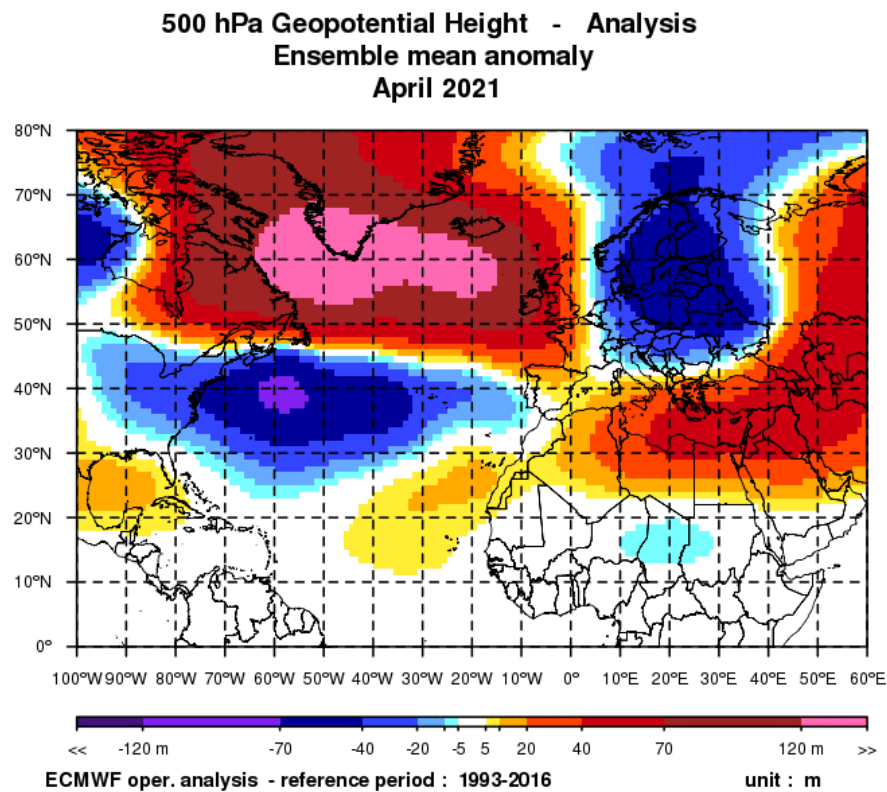
Figure 2.3: Anomalies of Geopotential height at 500hPa (Météo-France)
