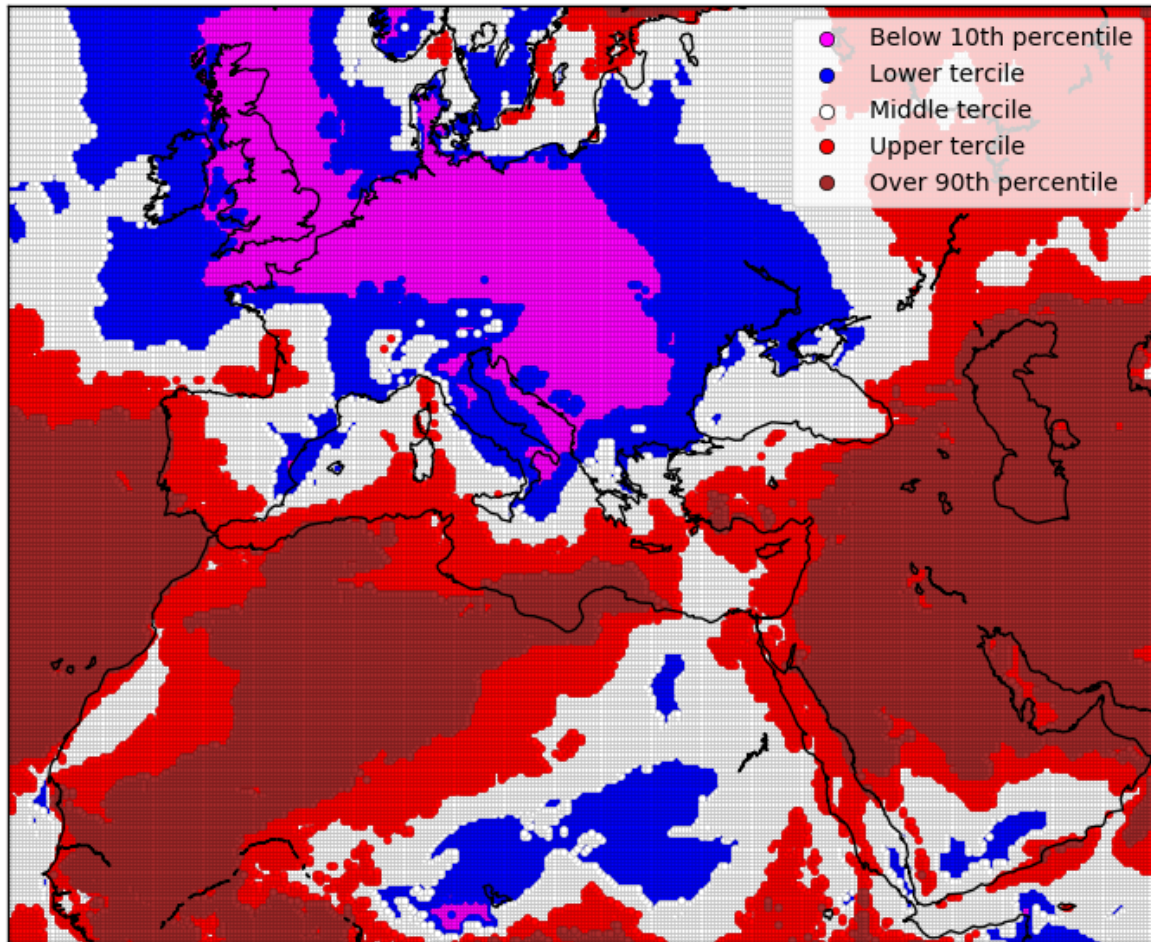
Observed categories (ref. 1981-2010) ['April'] 2021
