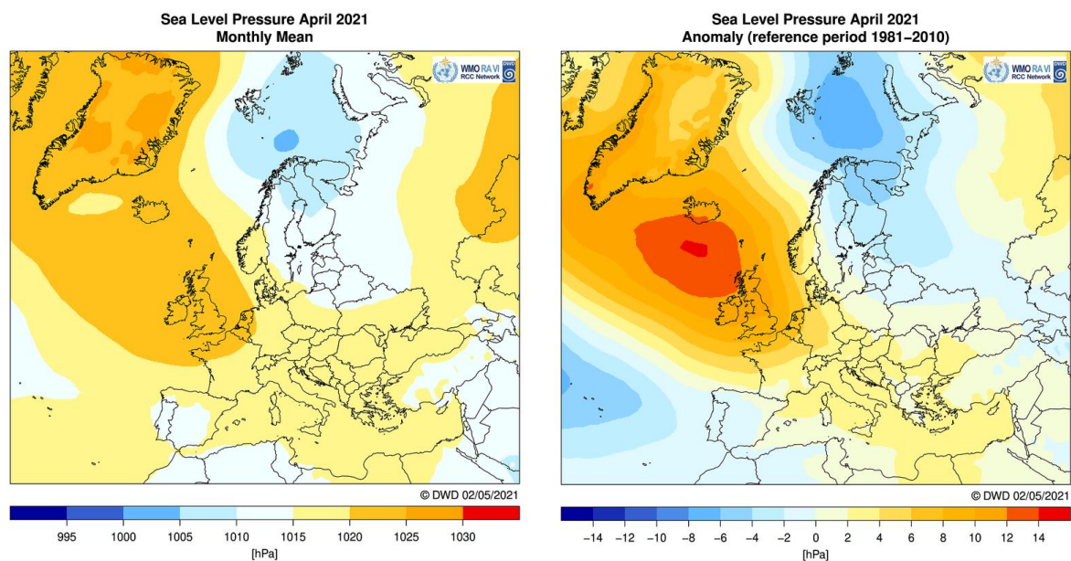
Figure 2.4: Mean sea level pressure over the North Atlantic, Europe and North Africa and 1981-2010 anomalies for April 2021. Source: DWD, https://www.dwd.de/DE/leistungen/rcccm/int/rcccm_int_ppp.html?nn=490674
