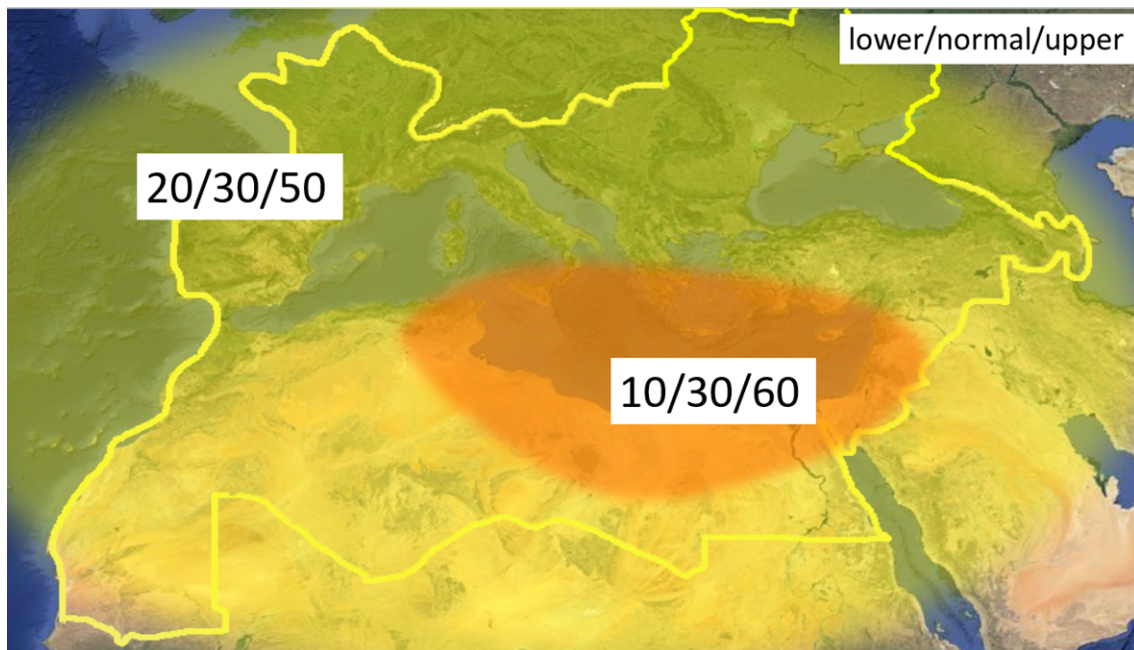
Figure 1. Graphical presentation of the 2024 summer temperature outlook. The maps show the probabilistic consensus forecast for tercile categories of anomalies for seasonal mean temperature, relative to the period 1991-2020. Due to the climate warming trend, anomalies are affected by the selected reference period.
