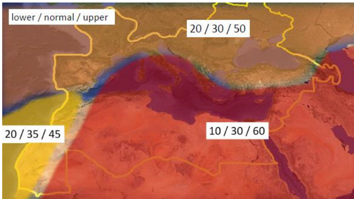
Figure 1. Graphical presentation of the 2017 summer temperature outlook. The maps show the probabilistic consensus forecast for tercile categories of anomalies for seasonal mean temperature, relative to the period 1981-2010. Due to the climate warming trend anomalies are affected by the selected reference period.
